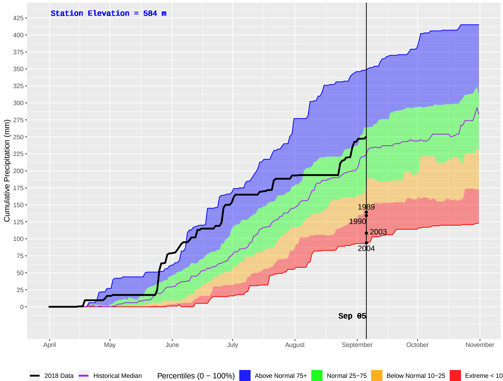
SIERRA (117) : Historical (1981–2016) and Current (2018) Daily Cumulative Precipitation
